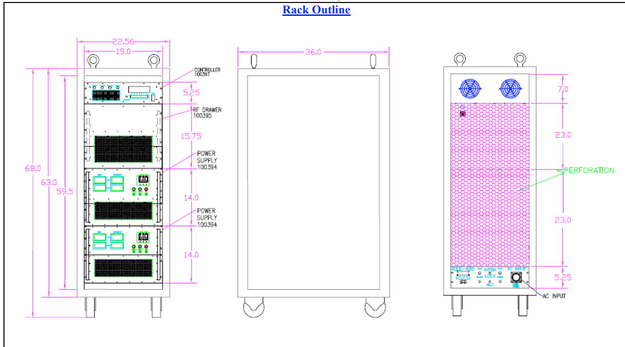
Rack Outline
